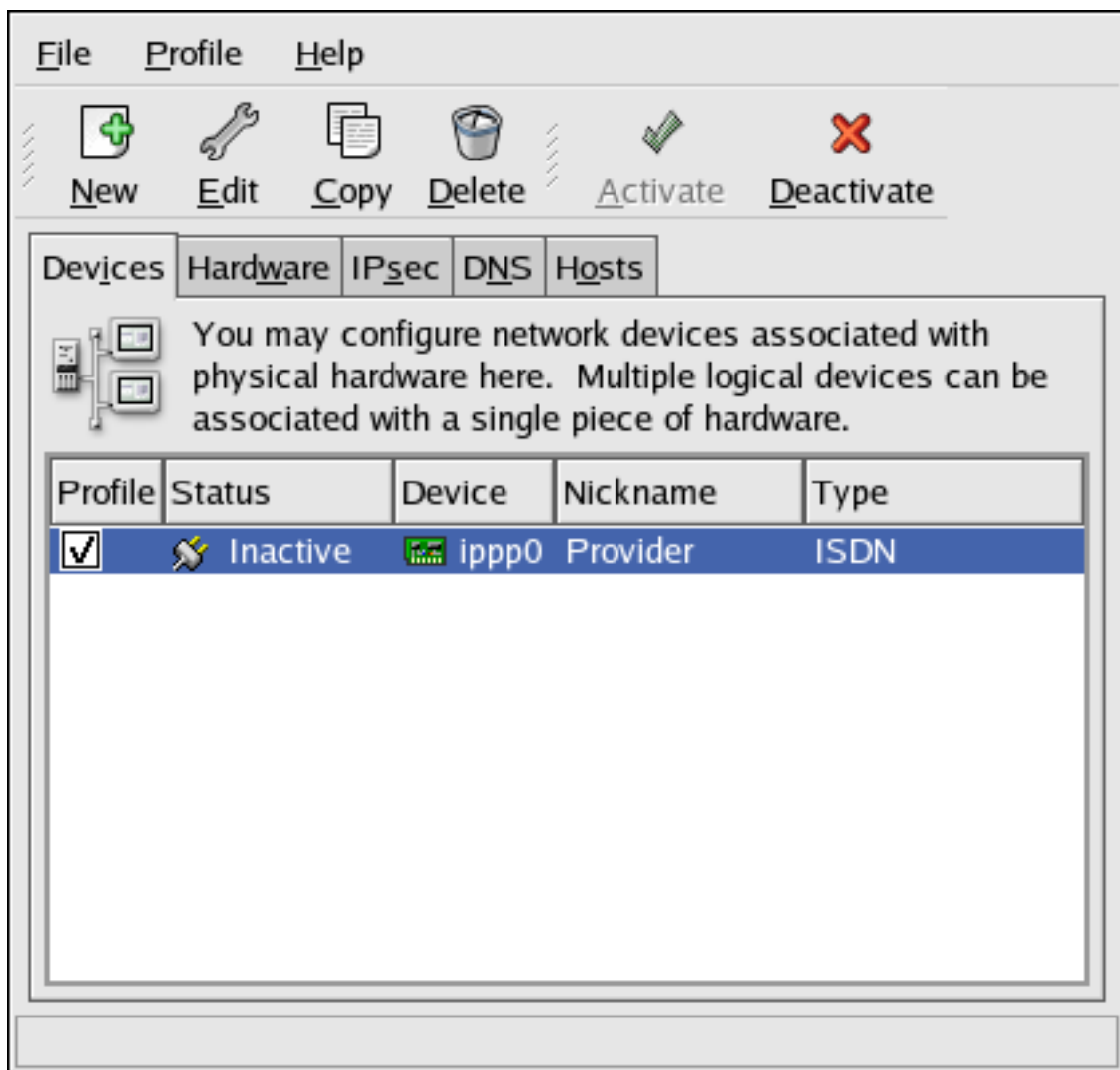
Figure 17.5. ISDN Device
