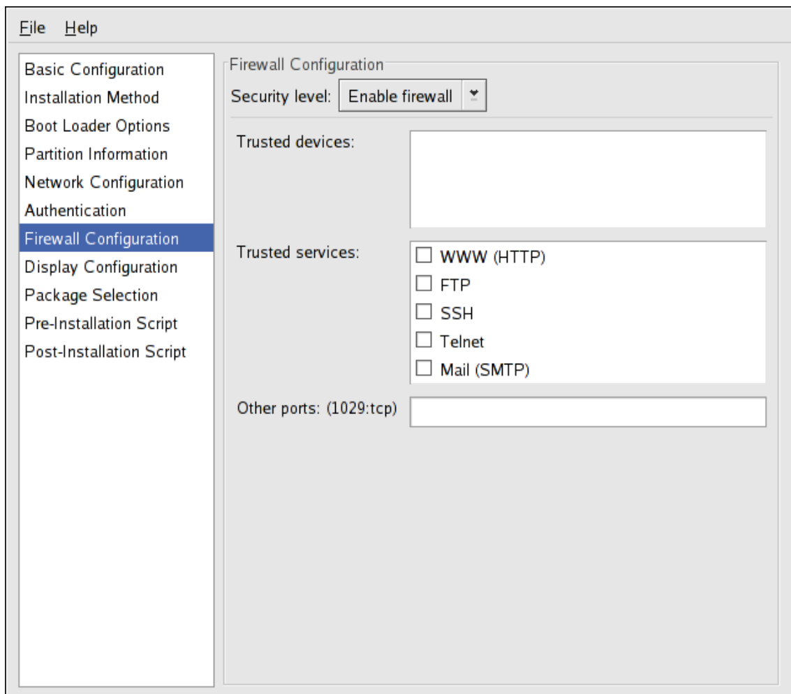
Figure 2.10. Firewall Configuration
