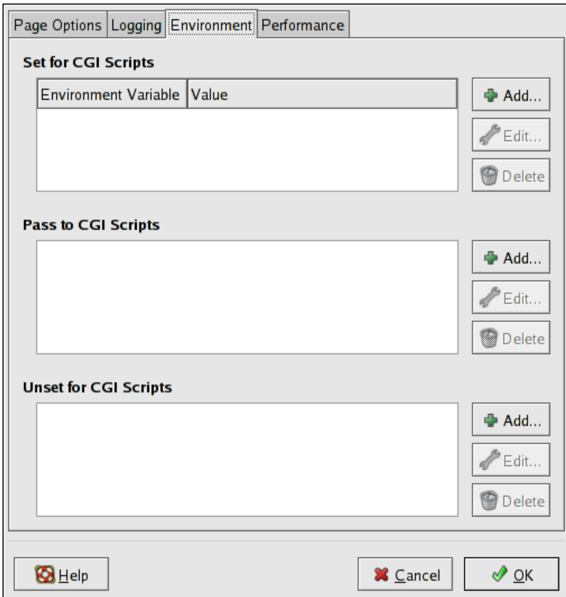
Figure 24.5. Environment Variables
