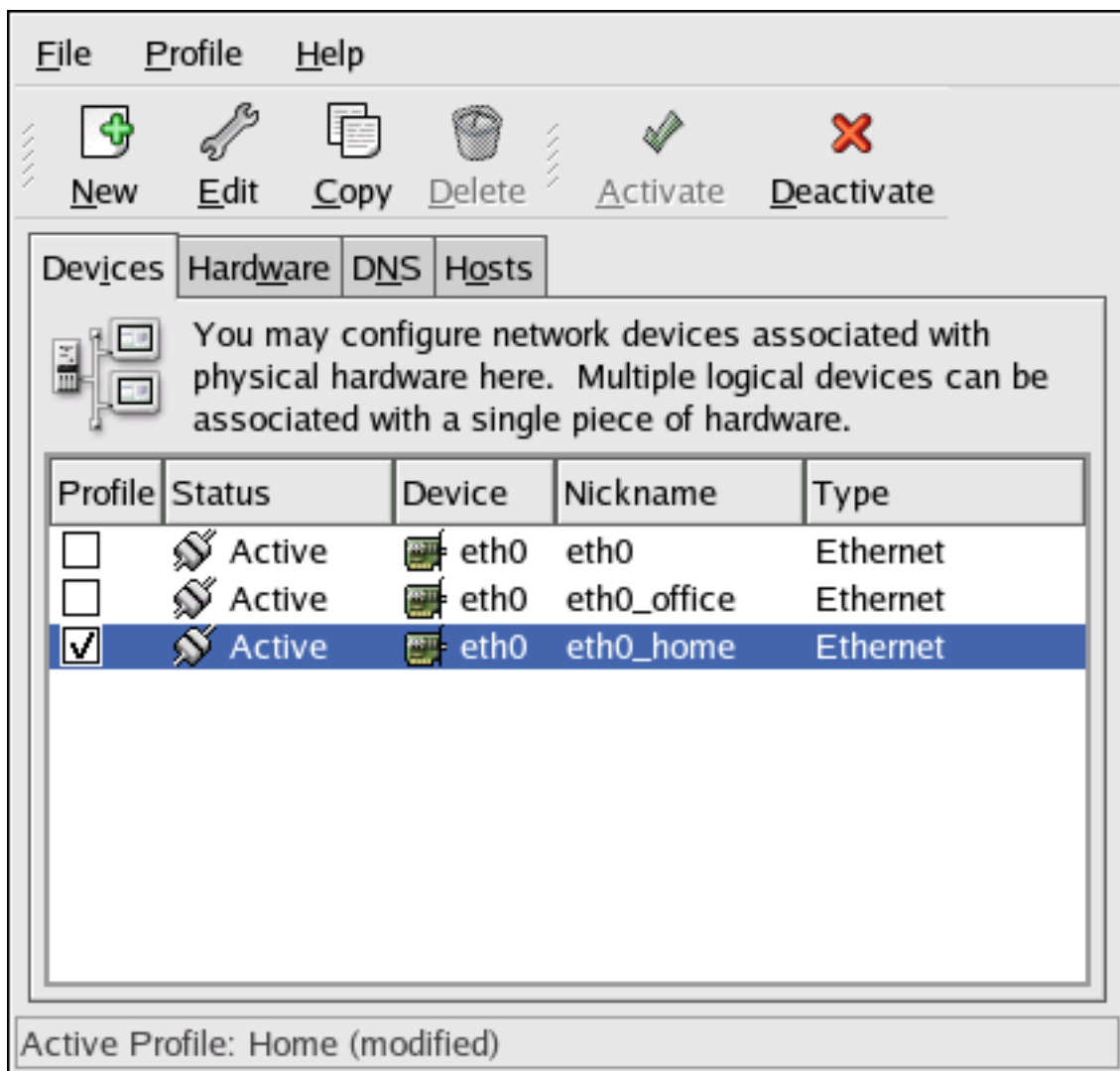
Figure 17.17. Home Profile
