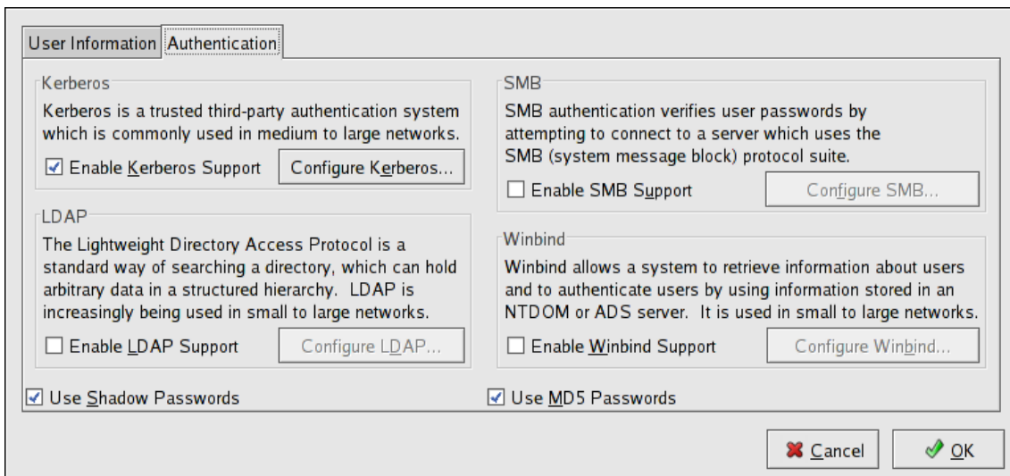
Figure 26.2. Authentication
