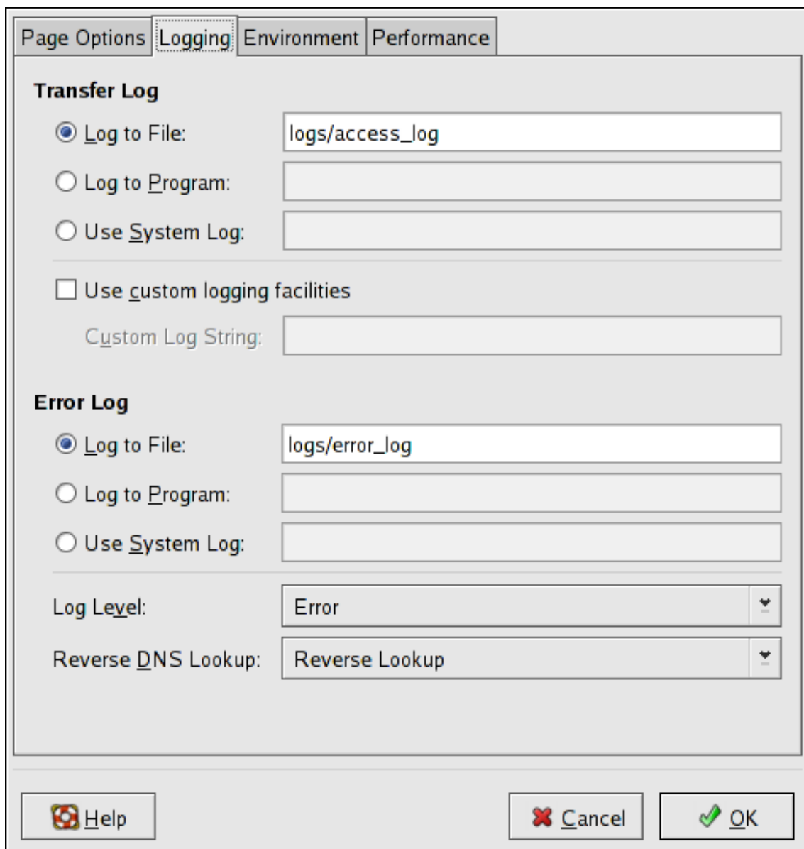
Figure 24.4. Logging
