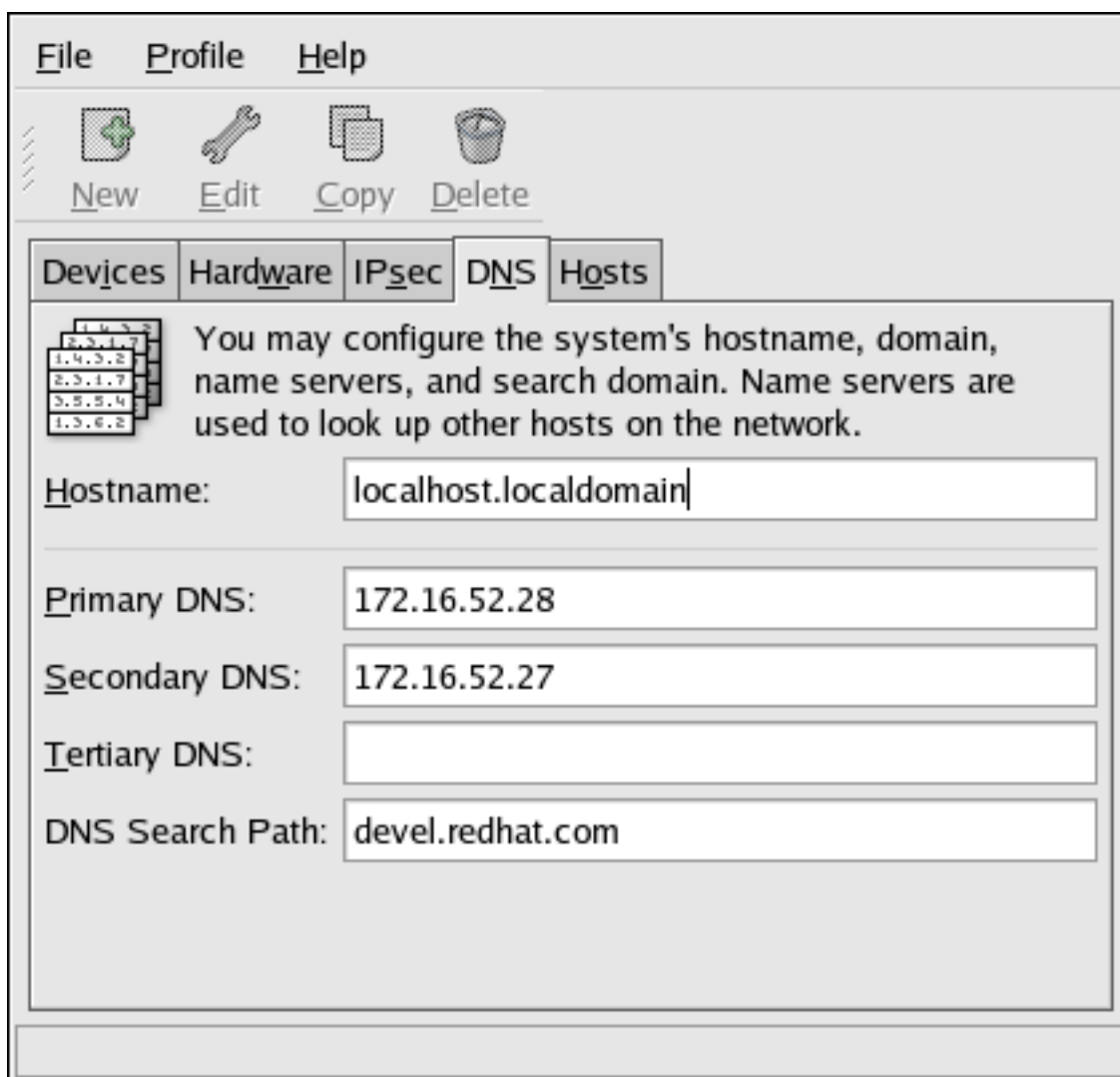
Figure 17.14. DNS Configuration
