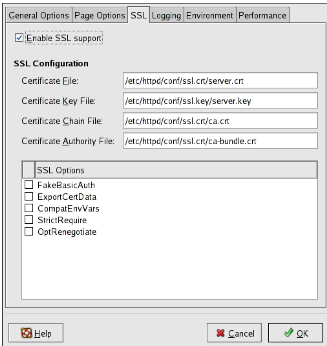
Figure 24.9. SSL Support
