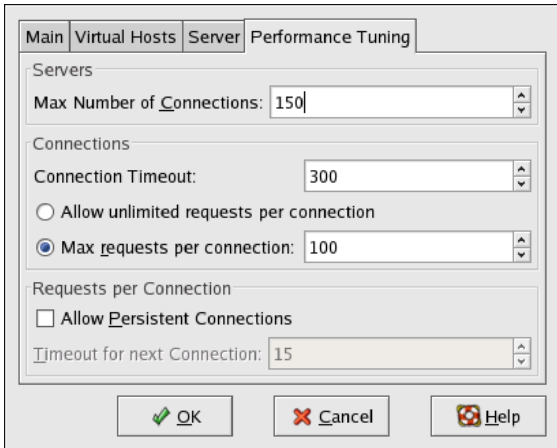
Figure 24.11. Performance Tuning
