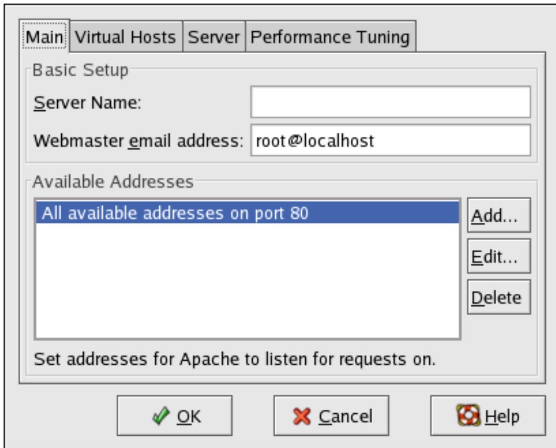
Figure 24.1. Basic Settings
