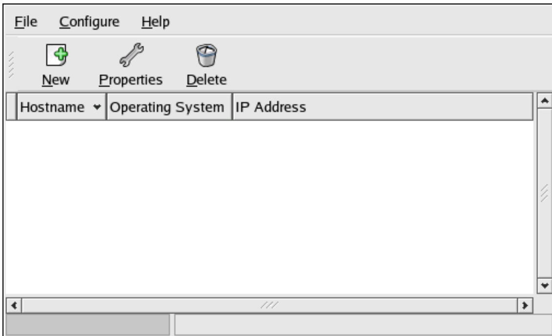
Figure 3.2. Add Hosts
