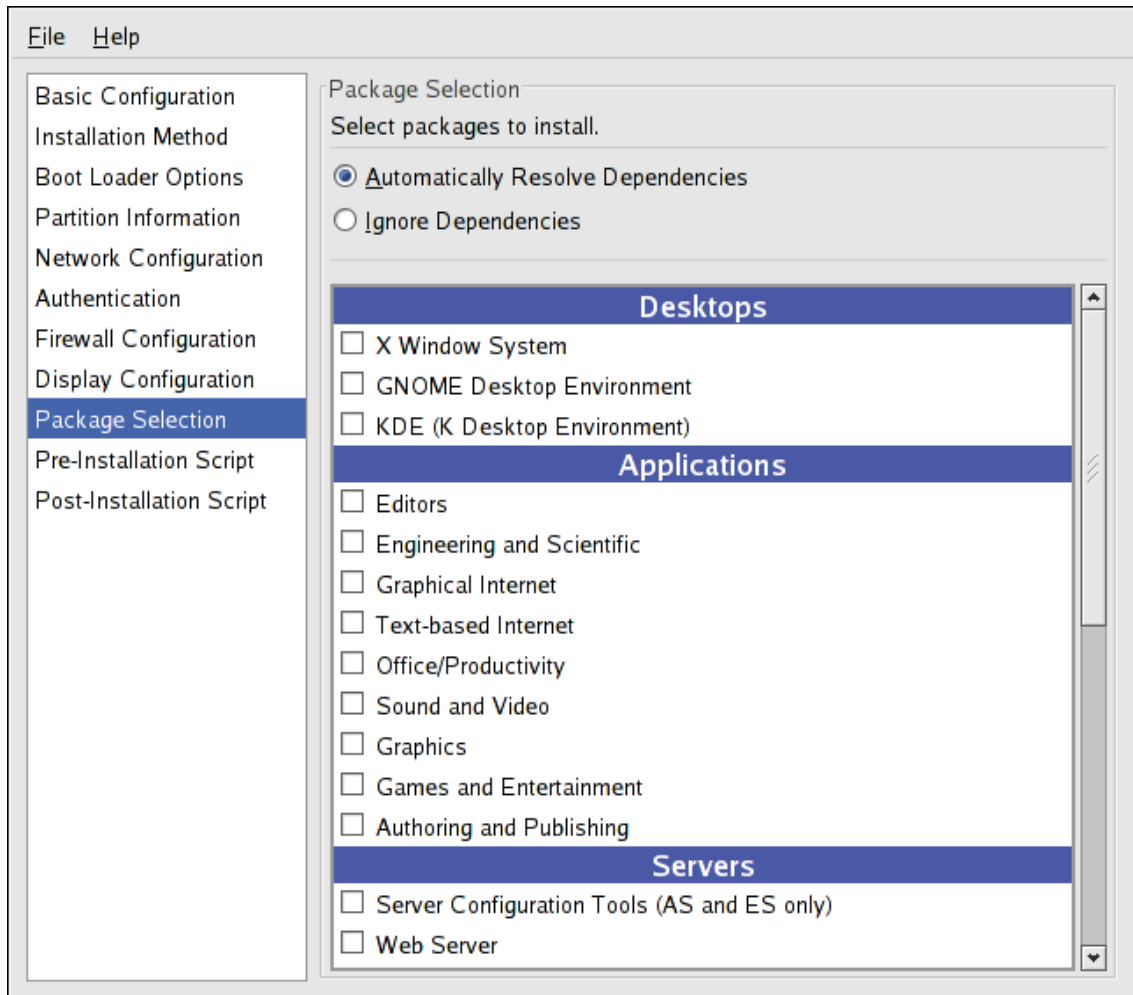
Figure 2.14. Package Selection
