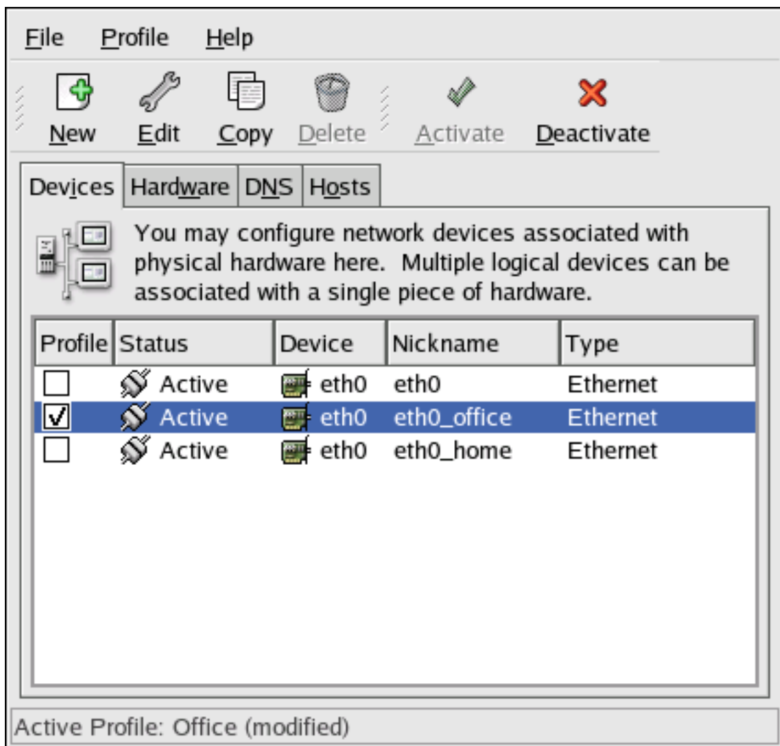
Figure 17.16. Office Profile
