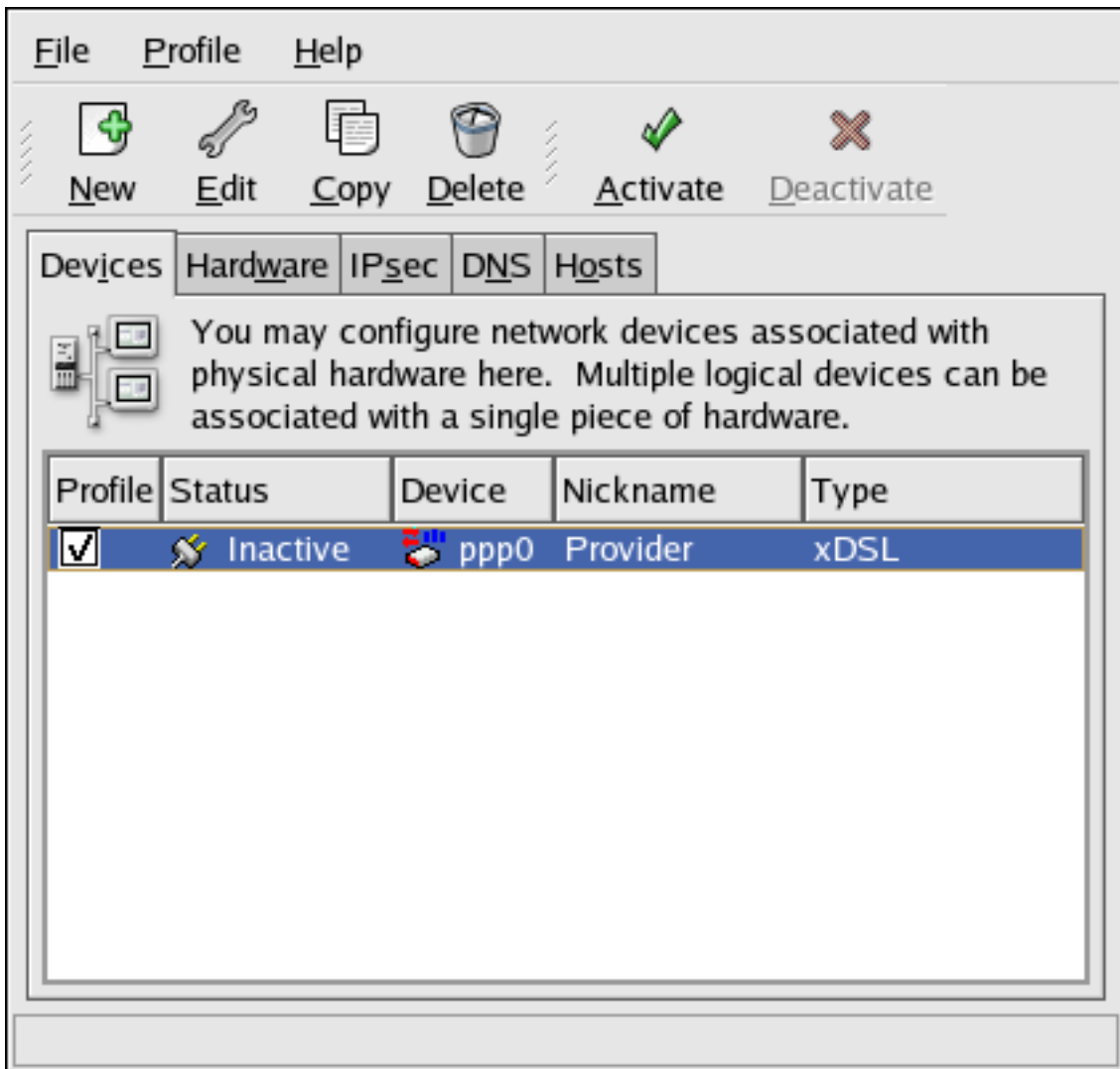
Figure 17.9. xDSL Device
