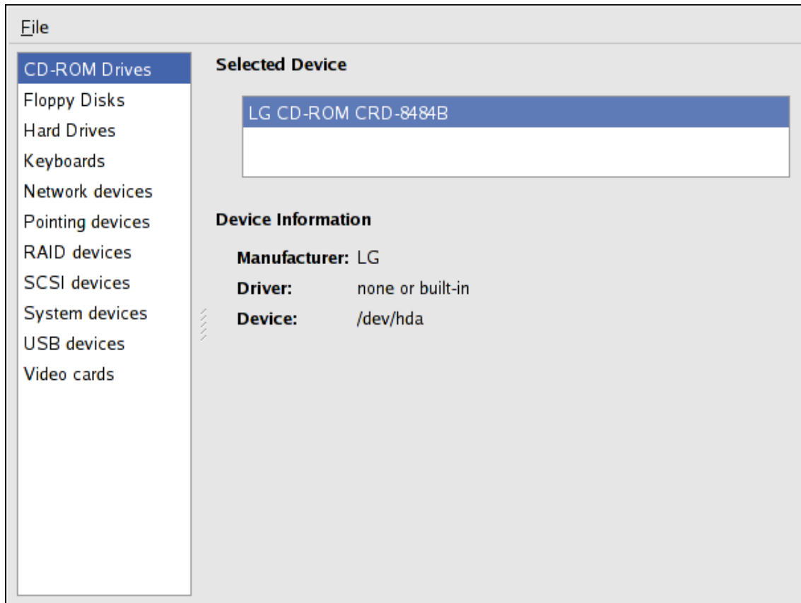
Figure 39.4. Hardware Browser
