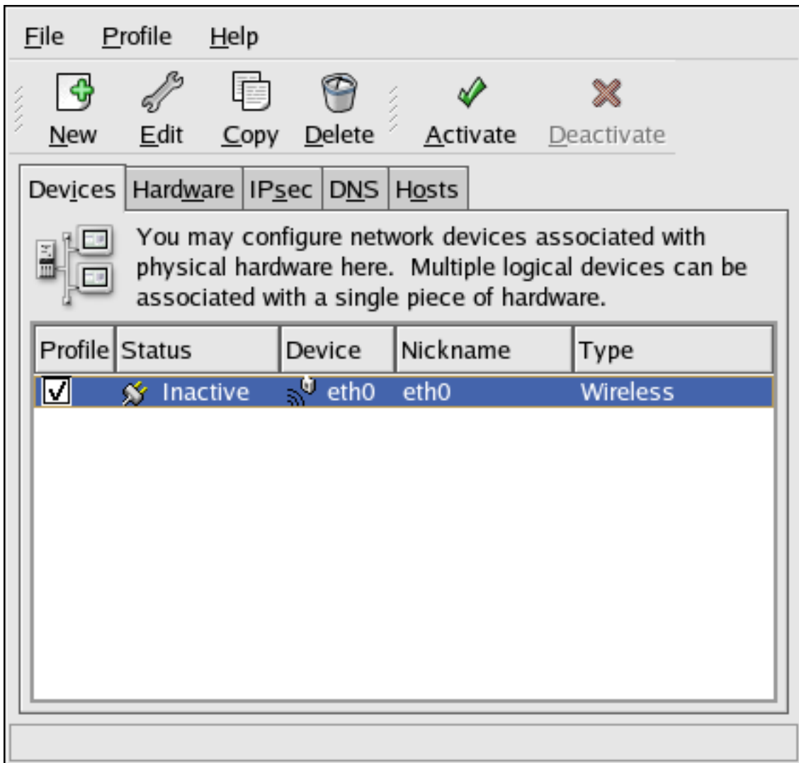
Figure 17.13. Wireless Device
