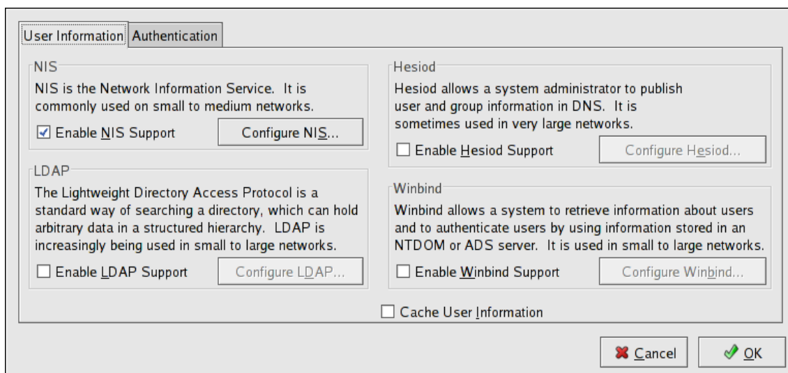
Figure 26.1. User Information
