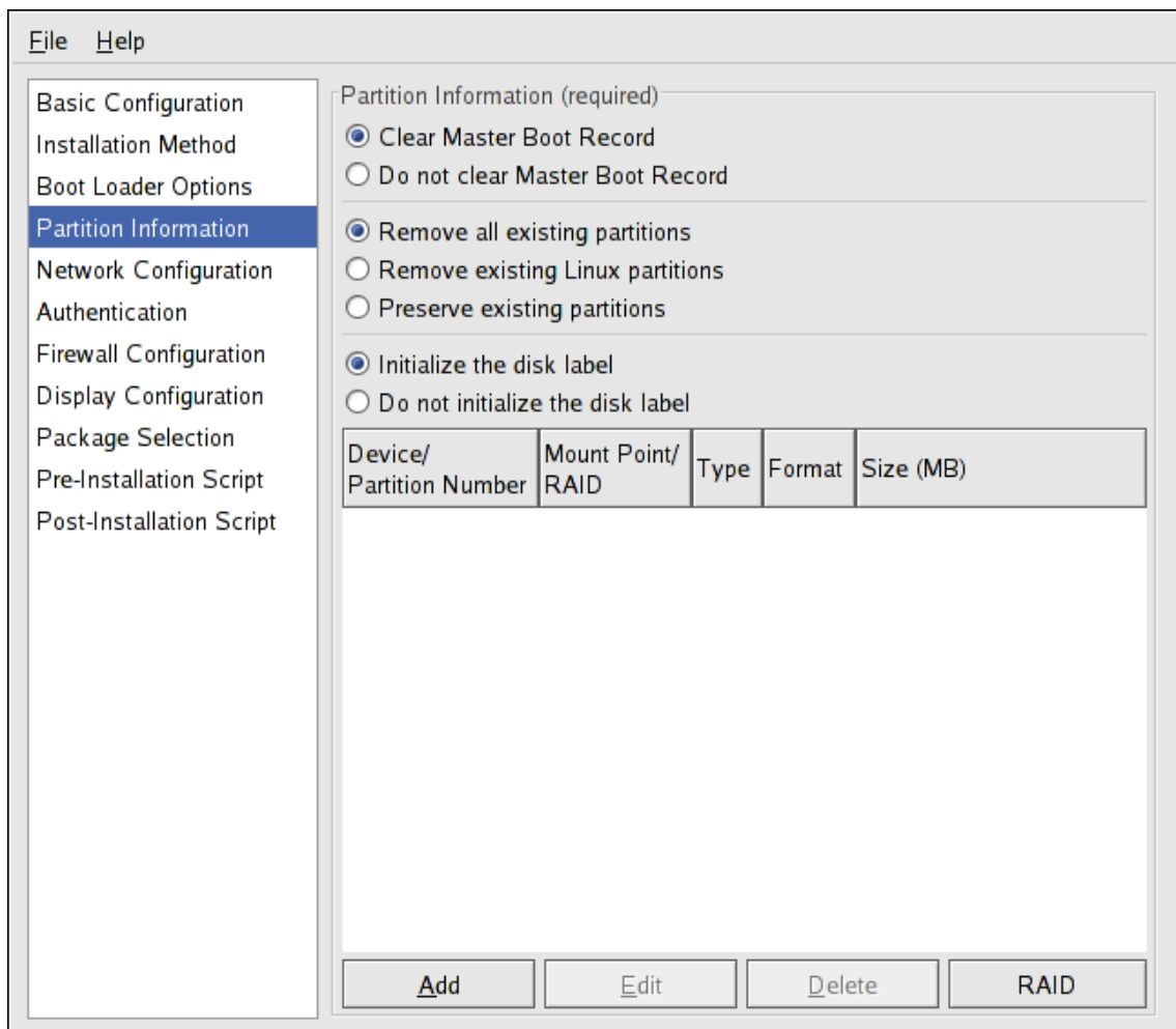
Figure 2.4. Partition Information
