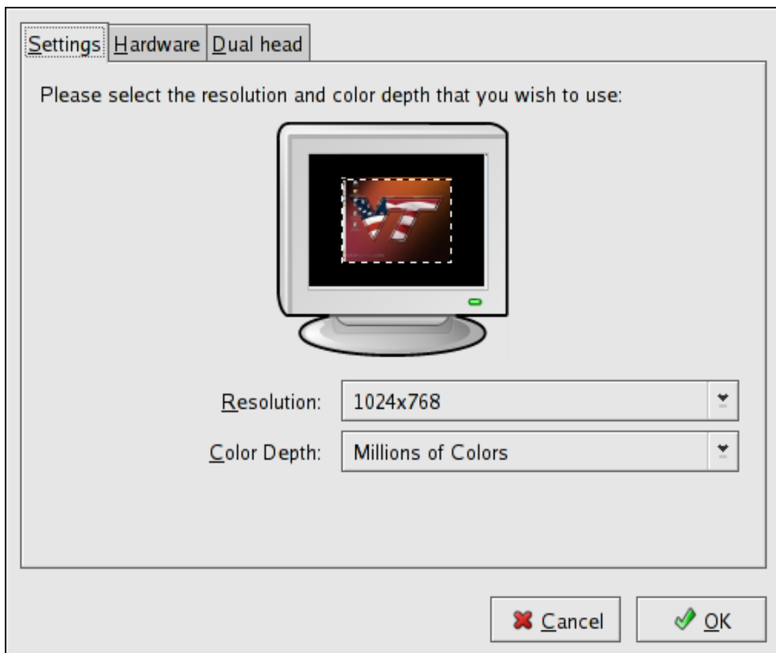
Figure 31.1. Display Settings
