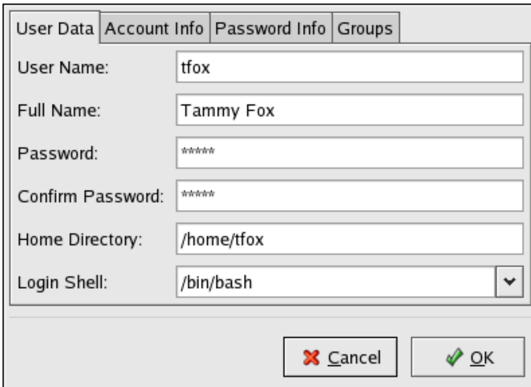
Figure 32.3. User Properties
